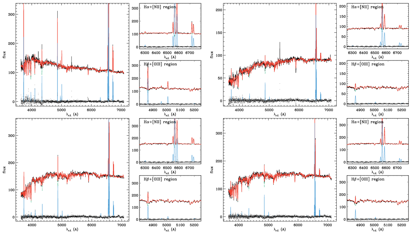
Figure 6. The SDSS spectra of four blue early-type galaxies processed with GANDALF . For each galaxy, we show the whole galaxy spectrum in the rest frame. The best fit is overlotted in red, while the fit to the emission lines is shown in blue. The residuals for this fit are also shown by the small points at the lower end of each panel, where the dashed lines further show the average level of the residuals that is used to assess the detection of the emission lines. We further focus in on two wavelength regions of interest around H\alpha+[NII] and H\beta+[OIII] . All four spectra feature deep Balmer absorption lines and some show considerable dust extinction.
