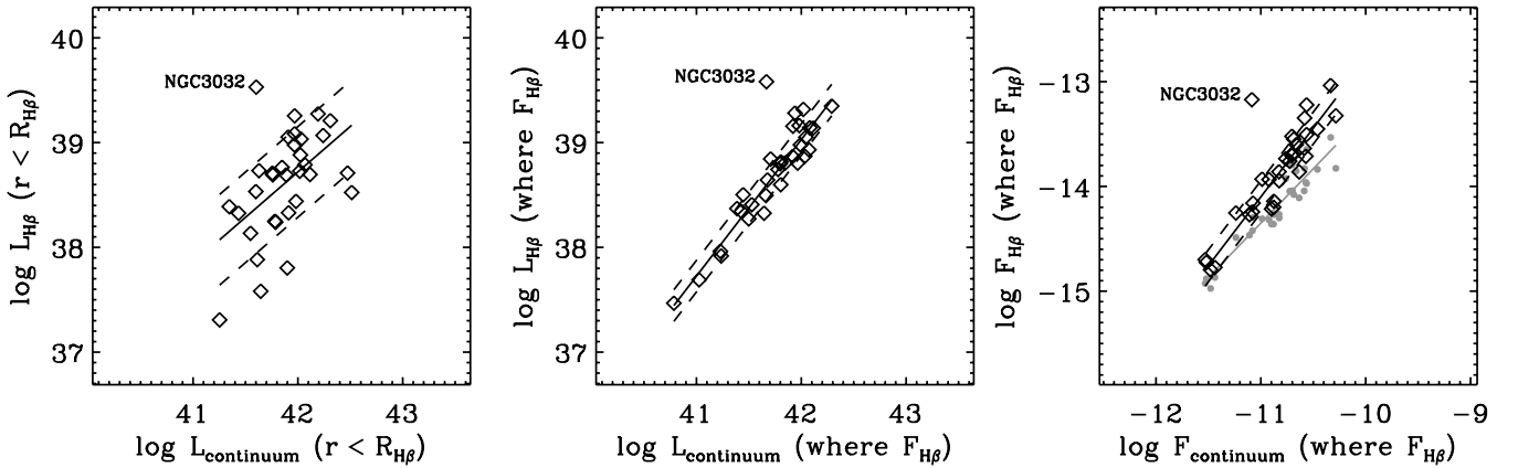
Figure 7. The connection between the integrated luminosity of the nebular emission and that of the stellar continuum in early-type galaxies. Left-hand panel: correlation between the luminosity of the stellar continuum L_{\text{cont}} and that of the \text{H}\beta emission L_{\text{H}\beta} observed in the SAURON spectra when both quantities are integrated within the average radius of the emission-line regions detected in each of our sample galaxies. The solid and dashed line show the best-fitting power-law fit to the observed distribution and associated 1\sigma scatter, respectively. Middle panel: same as left but now the total \text{H}\beta luminosity is juxtaposed to the stellar luminosity integrated only where the nebular \text{H}\beta emission is detected. A much tighter correlation emerges in this case. Right-hand panel: same as middle but now showing the correlation between the integrated nebular and stellar fluxes. A tight correlation persists, indicating that the L_{\text{cont}} - L_{\text{H}\beta} relation is not driven by the distance distribution of our sample galaxies. The light grey points show the integrated \text{H}\beta detection limits in each galaxy. Their position and alignment differ significantly from that of our integrated \text{H}\beta fluxes, dispelling also any doubts that the observed correlations are due to the limited range of our equivalent width sensitivity. In all panels, the position of NGC 3032, our most significant outlier, is indicated, and can be explained in terms of intense star formation activity.
