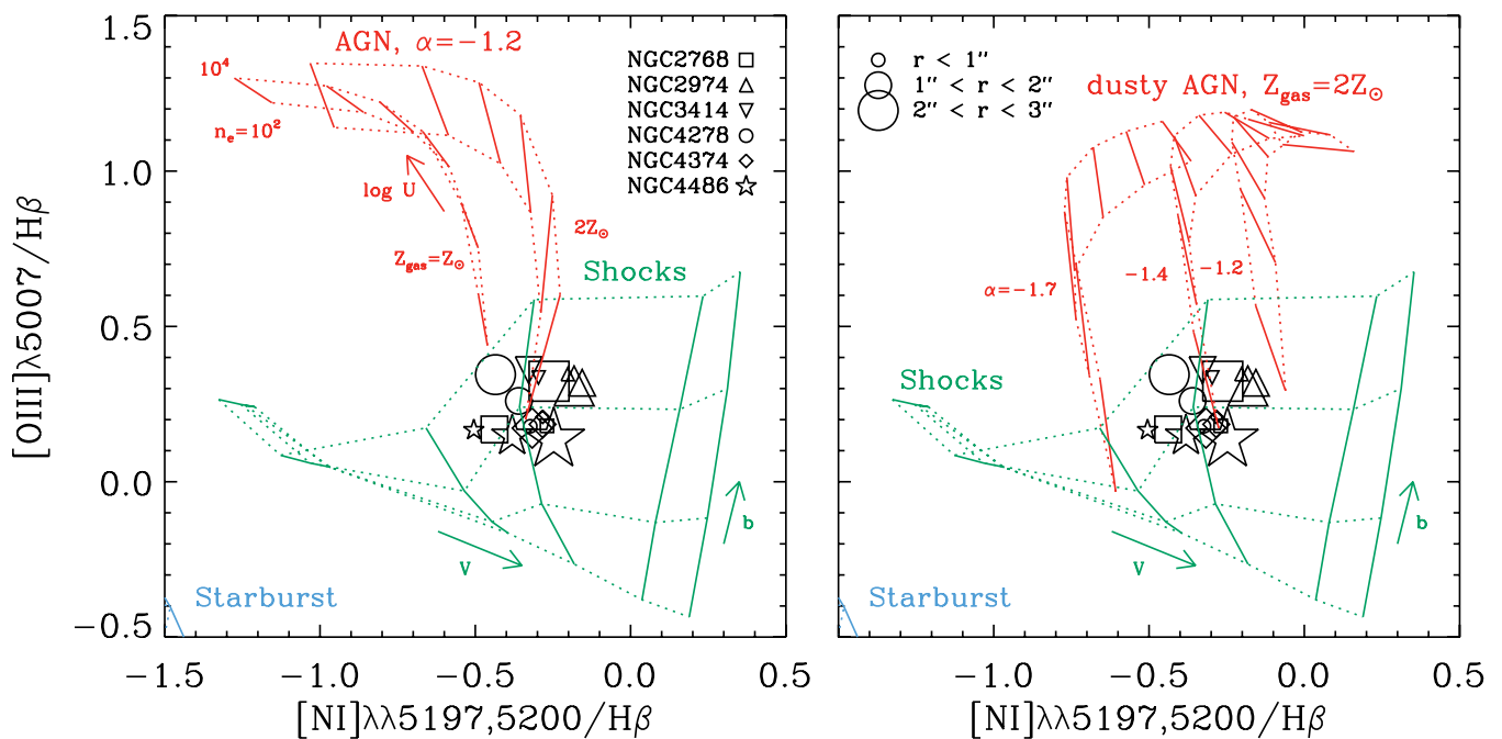
Figure 5. SAURON [\text{N I}]/\text{H}\beta versus [\text{O III}]\lambda 5007/\text{H}\beta diagnostic diagram for galaxies with 1.4-GHz radio cores. The different symbols correspond to each of the galaxies with detected [\text{N I}] emission, and the size of the symbols indicate the radial range over which the average values of the [\text{N I}]/\text{H}\beta and [\text{O III}]/\text{H}\beta ratios have been computed. The coloured grids show the same MAPPINGS-III models as in Fig. 1, except for the AGN photoionization models shown in the left-hand panel, which do not include dust, correspond to a single value of the power-law index of the AGN continuum of \alpha = -1.2 and are shown also for solar values of the gas metallicity. The range of the dimensionless ionizing parameter of the dust-free AGN models is also somewhat different, including values of \log U = -3.3, -3.0, -2.6, -2.3, -2.0, -1.6 .
