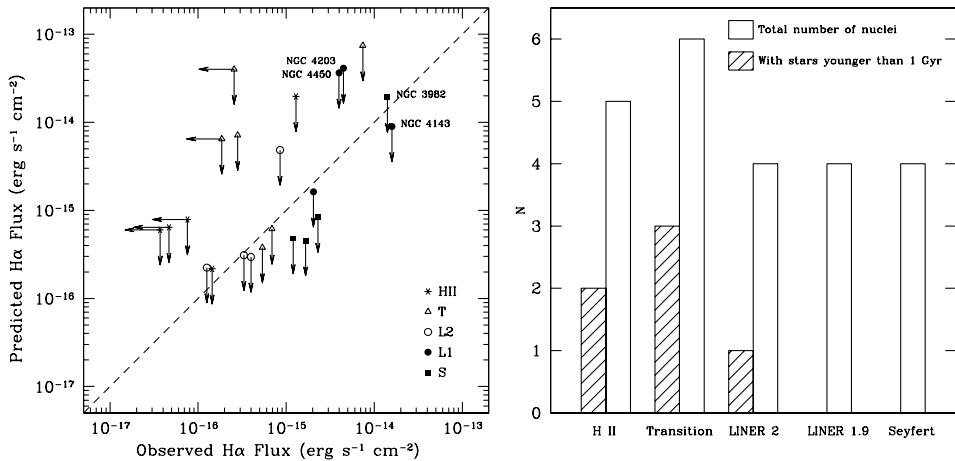
Figure 2. Left: Comparison of the H \alpha fluxes predicted for HII regions powered by the maximum number of young stars indicated by our G430L spectra, and the observed H \alpha emission in our G750M spectra. The symbol type denotes the ground-based, nuclear emission-line classification of our objects, while the dashed line shows the unity, consistency limit. Sources in which the stellar fluxes are probably overestimated due to contamination by an AGN continuum are labeled (NGC 3982, NGC 4143, NGC 4203, and NGC 4450). Correction of the observed H \alpha emission for internal extinction inferred from the observed decrement of the Balmer emission lines will further shift most plotted points to the right. Considering that emission-line fluxes obtained in ground-based measurements (Ho et al. 1997) contain 10–100 times as much emission as measured here, none of these galactic nuclei contain enough very young stars in their central \sim 10 pc to explain the nebular luminosity observed over \sim 100 pc scales. Right: Incidence of stars younger than 1 Gyr in the surveyed galactic nuclei as a function of their ground-based spectral classification.
