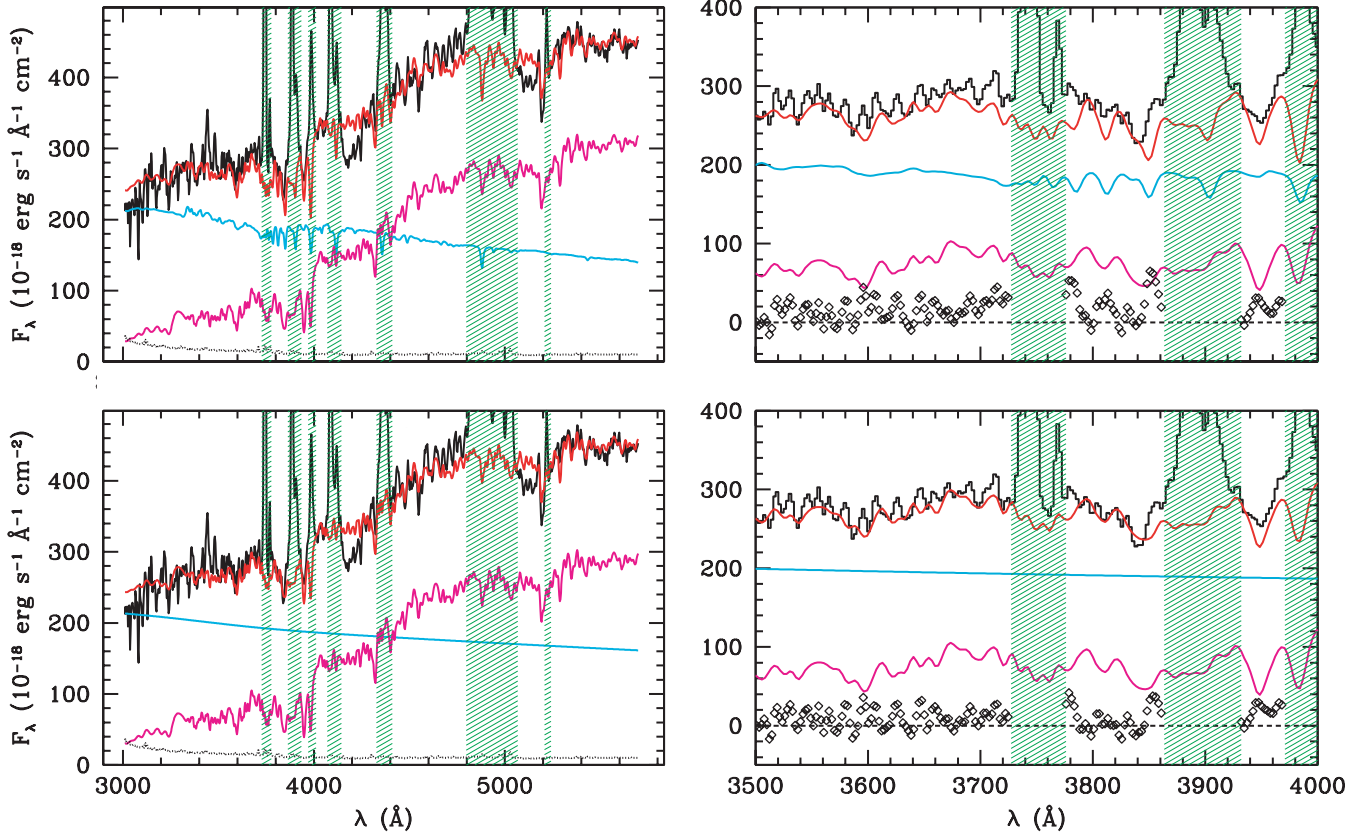
FIG. 6.—Young stars vs. AGN continuum in NGC 4203. Left : Same as Fig. 1, but now also showing separately the contribution of intermediate to old populations ( purple lines ) and of either young stars (<100 Myr; top, light blue lines ) or of the best power-law continuum ( bottom, light blue lines ). Both young stars and featureless continuum are allowed to be subject to a different amount of dust extinction than the rest of the stellar population. Right : Same as left , but now showing the fits in the wavelength region on either side of the Balmer break, with the corresponding residuals ( diamonds ). The model with independently reddened young stars requires them to be subjected to a considerable amount of extinction ( A_V = 2.2 mag) and to contribute 55% of the light (from the 3.2 Myr old template). The model with an AGN continuum needs only 10 Gyr old stars in addition to a power law with slope \alpha = 1.3 reddened by A_V = 0.2 mag.
