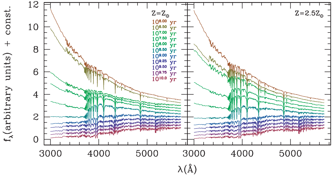
FIG. 2.—BC03 model SEDs for SSPs of different ages and solar ( left ) or 2.5 times solar ( right ) metallicities. The models are shown for the wavelength range matching our data, and for convenience of display they are normalized at 5700 Å and offset by a constant.
