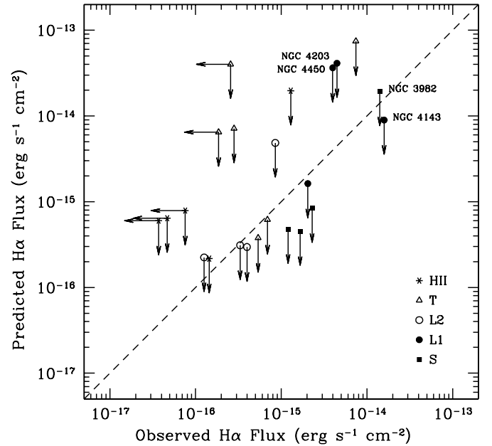
FIG. 9.—Comparison of the predicted H \alpha fluxes for H II regions powered by the maximum number of young stars indicated by our G430L spectra with the observed H \alpha emission in our G750M spectra. The symbol type denotes the ground-based nuclear emission-line classification of our objects, whereas the dashed line shows the unity and consistency limit. Sources in which the stellar fluxes are probably overestimated because of contamination by an AGN continuum are labeled (NGC 3982, NGC 4143, NGC 4203, and NGC 4450). Correction of the observed H \alpha emission for internal extinction inferred from the observed decrement of the Balmer emission lines shifts most plotted points farther to the right.
