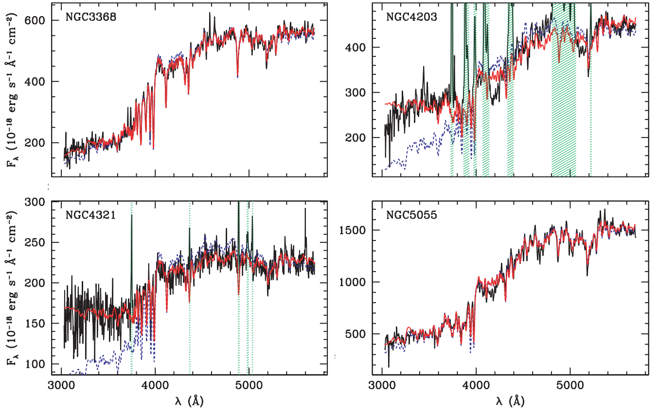
FIG. 4.—Examples of fits obtained with multiple-starburst models ( red lines ) vs. single-age models ( violet dashed lines ).
