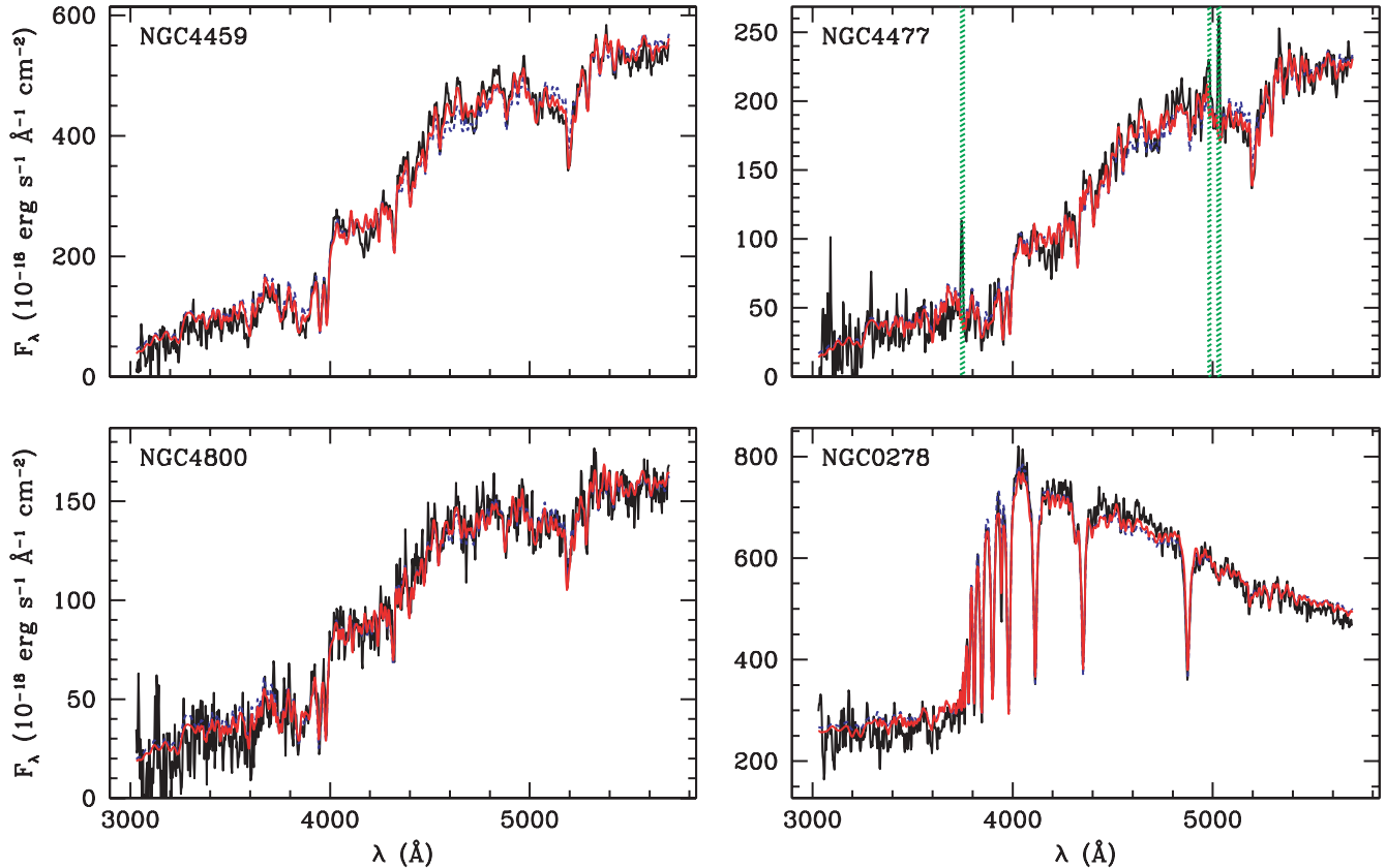
Fig. 7.—Examples of multiple-starburst models with supersolar ( Z = 2.5 Z_{\odot} ; red lines) or solar ( Z = 1 Z_{\odot} ; violet dashed lines) metallicity.
