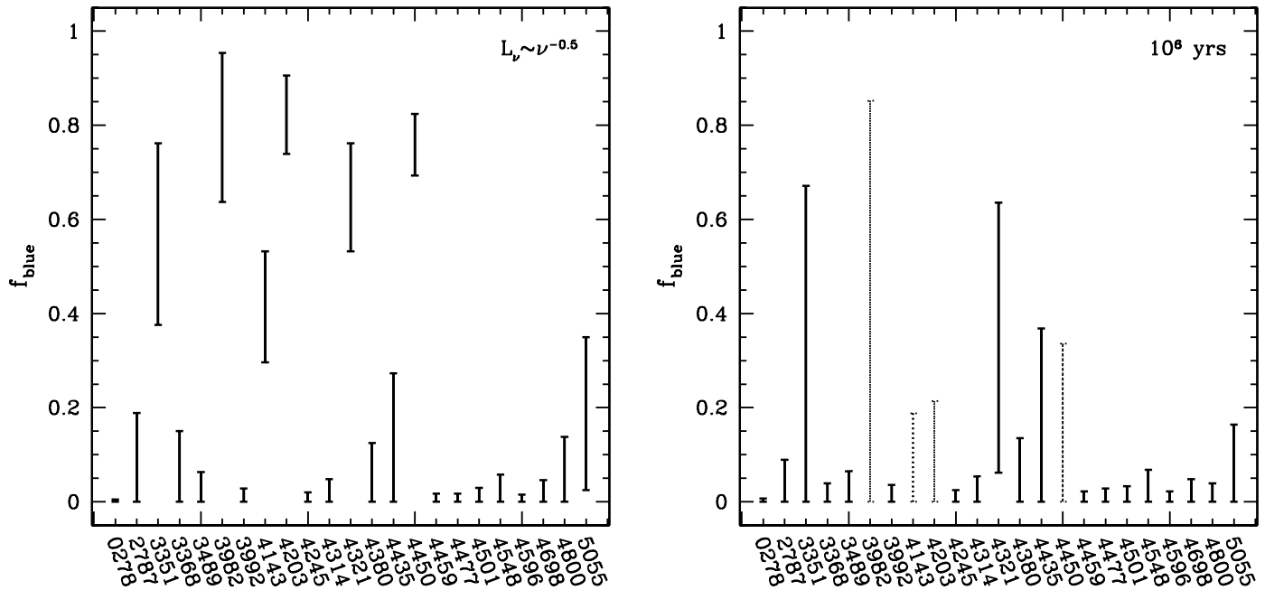
FIG. 8.— Confidence limits ( 3\sigma ) for the flux fraction in the range 3050–3200 Å from a power-law featureless continuum (for L_\nu \propto \nu^{-0.5} ; left ) or a single 10^6 yr old starburst population model ( right ). The dotted lines identify cases in which the need for young stars is most likely overestimated by the models of § 4.2. Each number on the abscissa is the NGC name of a galaxy.
