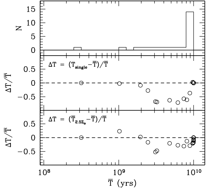
FIG. 3.—Distribution of the luminosity-weighted age estimates obtained from the best-fitting multiple-starburst models ( top ), compared with the age of the best single-age models of § 4.1 ( middle ) and the luminosity-weighted ages of § 4.3, from multiple-starburst models of supersolar metallicity ( bottom ).
