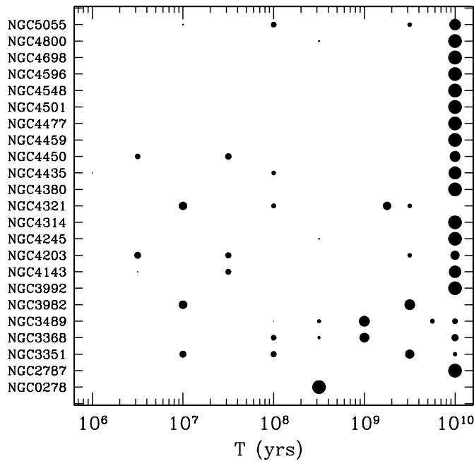
FIG. 5.—Graphical visualization of the relative light contribution of each single-age model to the best multiple-starburst models. The areas of the circles are directly proportional to the relative weights listed in Table 4.
