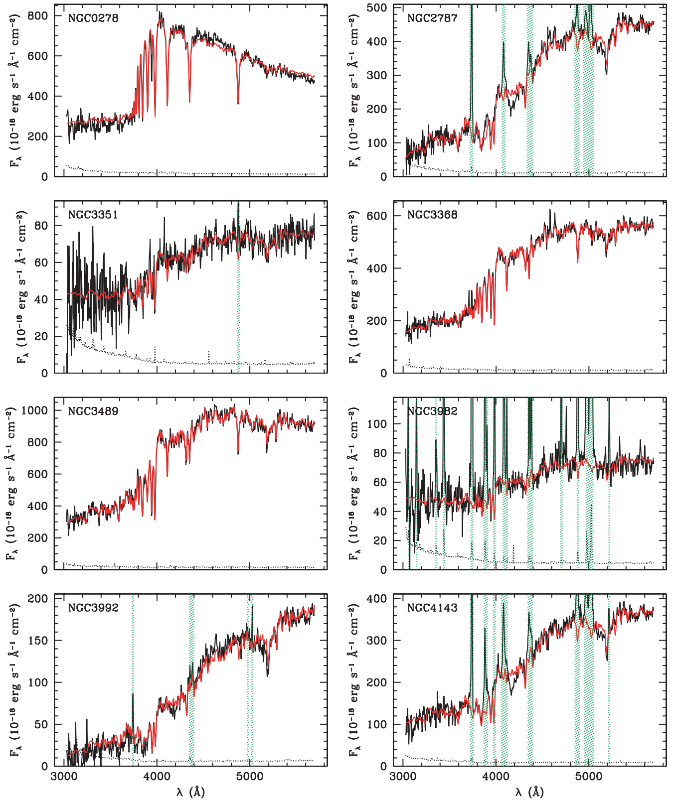
FIG. 1.—Nuclear G430L spectra extracted from the central 0''.25 \times 0''.2 of our sample galaxies. The dotted lines at the bottom of each plot show the error array corresponding to the observed fluxes, whereas the dashed green columns indicate the spectral regions excluded during our analysis to avoid emission lines. The red lines show our best-fitting multiple-starburst population models. The observed fluxes have been corrected for Galactic foreground extinction, whereas the models account for dust extinction intrinsic to the source.
