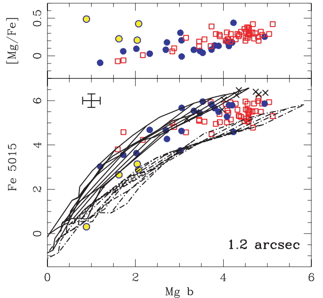
Figure 3. Bottom: index–index diagram showing central line indices Mg\ b and Fe\ 5015 (in \text{\AA} ) in circular apertures with radius 1.2 arcsec for the Sa galaxies (in blue, with representative error bars), together with integrated indices within r_e/8 for the early-type galaxies of paper VI (in red), and with SSP stellar population models by Thomas et al. (2003). Here models are plotted with [Mg/Fe] = 0 (solid lines) and 0.5 (dashed–dotted), ranging in metallicity from Z = -2.25 to 0.35 and in age from t = 0.1 to 15 Gyr. The models with the highest metallicity ( Z = 0.35 ) and age (15 Gyr) have the highest Mg\ b and Fe\ 5015 values. The black crosses are the central values for the 10 spiral galaxies of Proctor & Sansom (2002), for which they claim to have reliable corrections for H\beta emission. Top: [Mg/Fe] ratios calculated from the \chi^2 code (Paper VIII), calculated assuming the stellar populations can be represented by an SSP. The four blue points filled in yellow are NGC 1056, 2273, 4383 and 5953, objects with large central H\beta values, that most likely cannot be fitted with SSP models.
