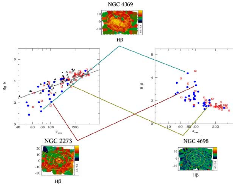
Figure 7. Same as Figs 5 and 6, but now with H\beta maps of three example galaxies, which show that the stellar populations are young when the galaxies lies off the relation for galaxies in the Coma cluster.
