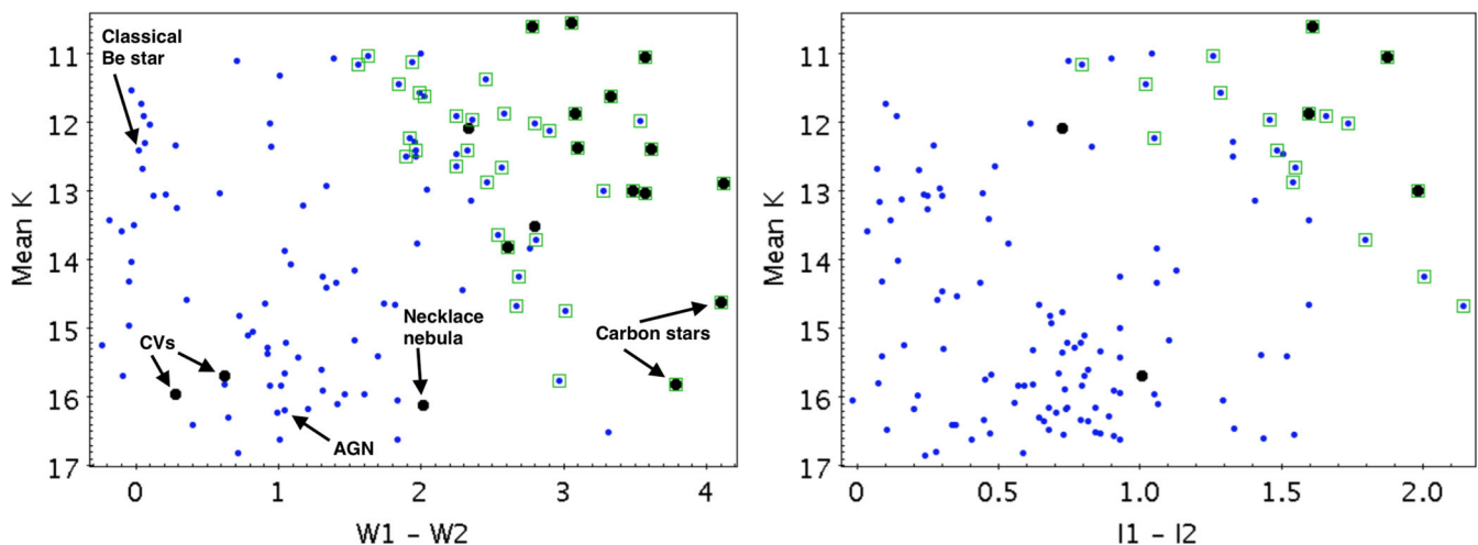
Figure 7. CMDs for non-YSOs. Left: mean UGPS K versus WISE W1–W2. Right: mean UGPS K versus Spitzer /IRAC I1–I2. The IRAC I1 and I2 data are a little deeper than WISE W1 and W2, but they do not cover the full area of the UGPS catalogue. Known variables are marked in black and variables in our dusty AGB star selection region in Fig. 8 are enclosed in green squares. Dusty AGB stars mostly found at the upper right. The nature of the small group of bright blue variable stars in the left-hand panel is unclear, see the text. The larger group of faint variables includes both faint red stars (some of which will be relatively isolated YSOs) and faint blue variables such as CVs, EBs and AGN, seen in greater numbers in the upper left panel of Fig. 5.
