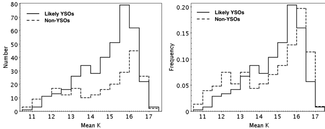
Figure 6. Mean UGPS K magnitude distributions for likely YSOs and non-YSOs. Left: absolute numbers. Right: normalized distributions, each with unit area.
