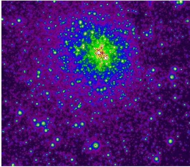
Figure 5. GPS K band image of obscured globular cluster GLIMPSE-C01.
